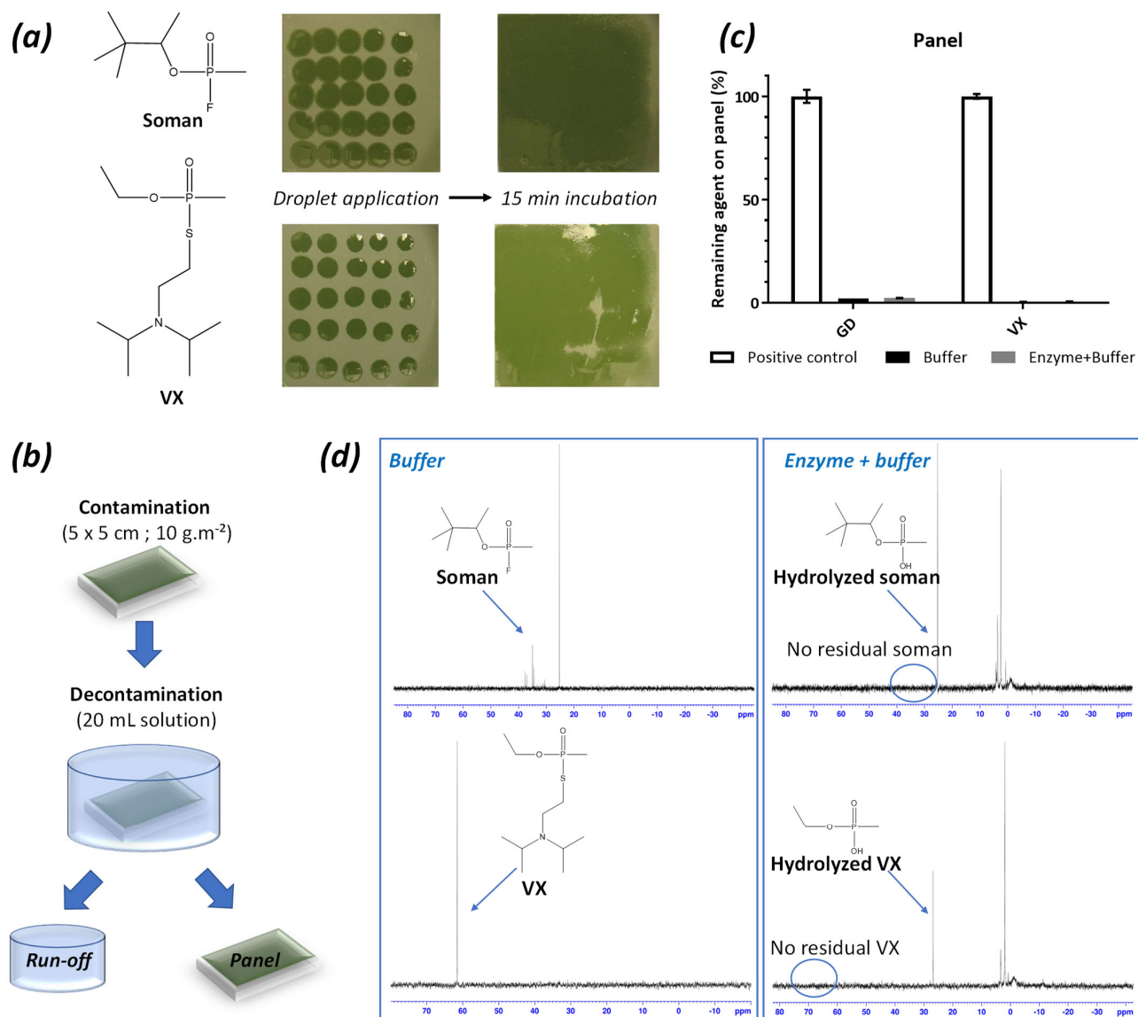
Figure 4. Enzyme decontamination of painted panels. (a) Contamination of panels with droplets of agent to reach a final contamination of 10 g·m -2 of soman or VX. (b) Contaminated panels (5 × 5 cm) are incubated for 15 min in 20 mL of decontamination solutions. (c) Evaluation of residual soman (GD) and VX on panels after decontamination. (d) Evaluating remaining soman and VX in liquid decontamination (run-off) solution.
