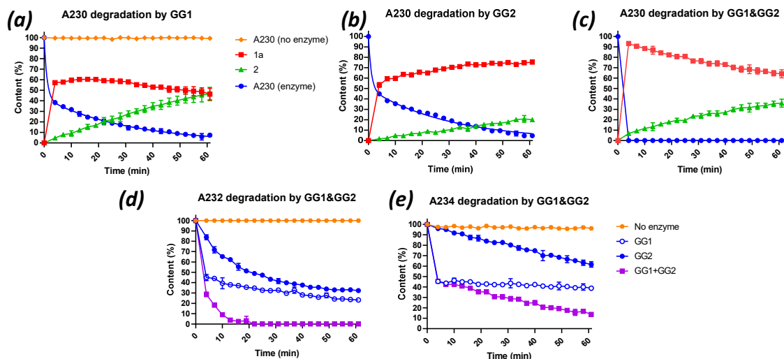
Figure 2. Degradation curves of Novichok agents A230, A232 and A234 by GG1 and GG2 enzymes. Degradation of A230 by GG1 (a) and GG2 (b) or both (c). Red and green represent the products of A230 hydrolysis. Degradation of A232 (d) and A234 (e) by GG1, GG2 or both. Agent concentration: 25 mM, enzyme concentration; 20 \mu M (for GG1 and GG2 mix, 1:1 ratio). Experiments were conducted in 100–200 mM Tris buffer pH 9, 50 mM NaCl at 23 ^{\circ} C.
