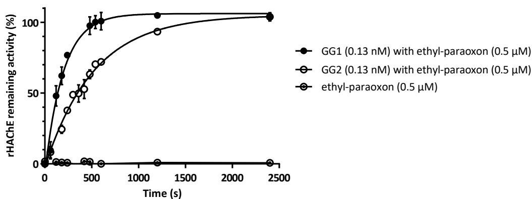
Figure 5. rHAcHE inhibition assay [50] with ethyl-paraoxon ( 0.5 \mu\text{M} ) previously incubated with GG1 or GG2 ( 0.13 \text{ nM} ) and control without PTE.
